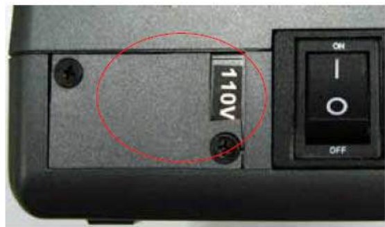
110VAC selected
